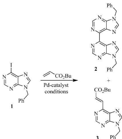
Scheme 1. Reaction between 9-benzyl-6-iodopurine and butyl acrylate under the conditions of the Heck reaction.
