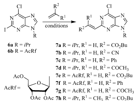
Scheme 3. Heck reactions of 6-chloro-2-iodopurine derivatives.
