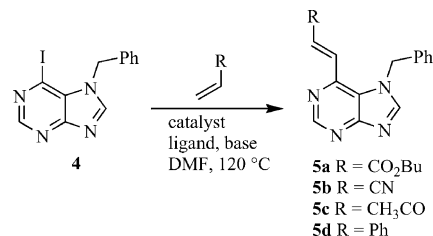
Scheme 2. Heck reactions of 7-benzyl-6-iodopurine.
